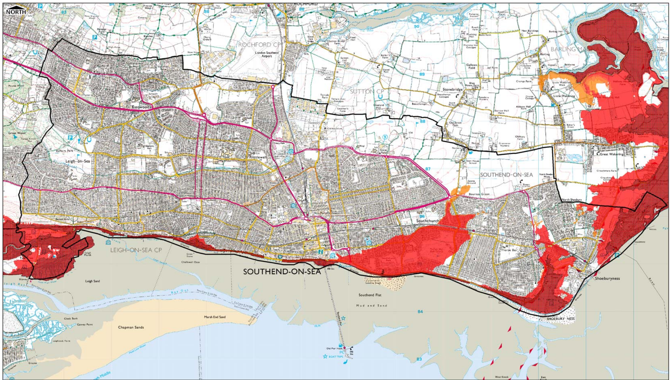
FIGURE C16 - COMPOSITE TIME TO INUNDATION (FROM BREACH EVENT) 1000YR 2110
