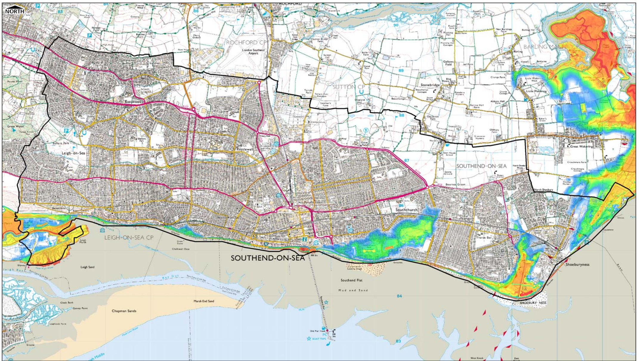
FIGURE C2 - COMPOSITE MAXIMUM FLOOD DEPTH 200YR 2110 (BREACH AND OVERTOPPING)
