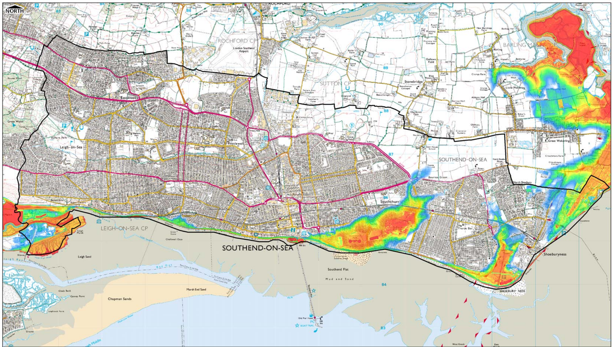
FIGURE C6 - COMPOSITE MAXIMUM FLOOD DEPTH 1000YR 2110 (OVERTOPPING)
