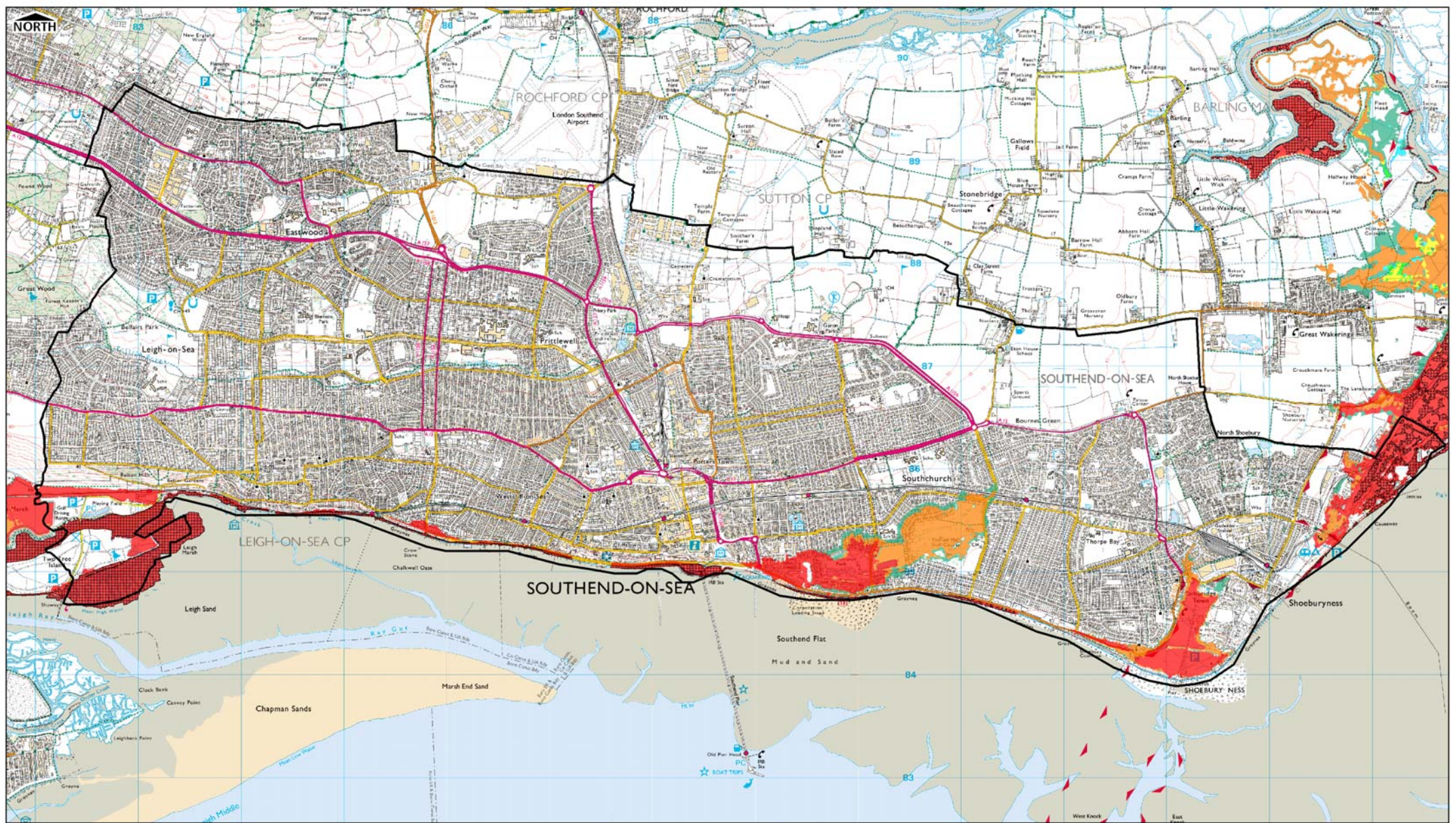
FIGURE C13 - COMPOSITE TIME TO INUNDATION (FROM BREACH EVENT) 200YR 2010
