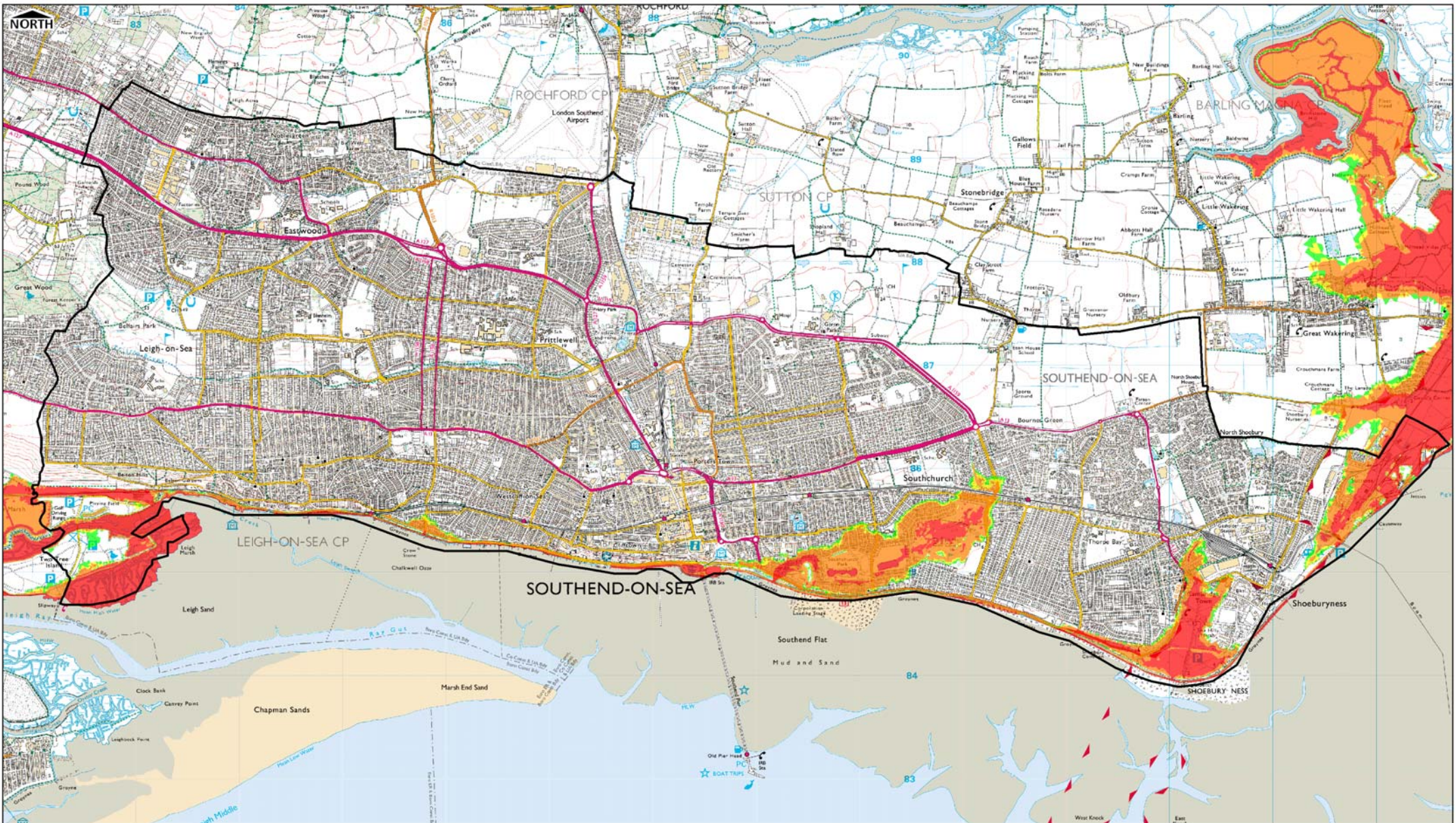
FIGURE C10 - COMPOSITE MAXIMUM HAZARD 1000YR 2010 (BREACH AND OVERTOPPING)
