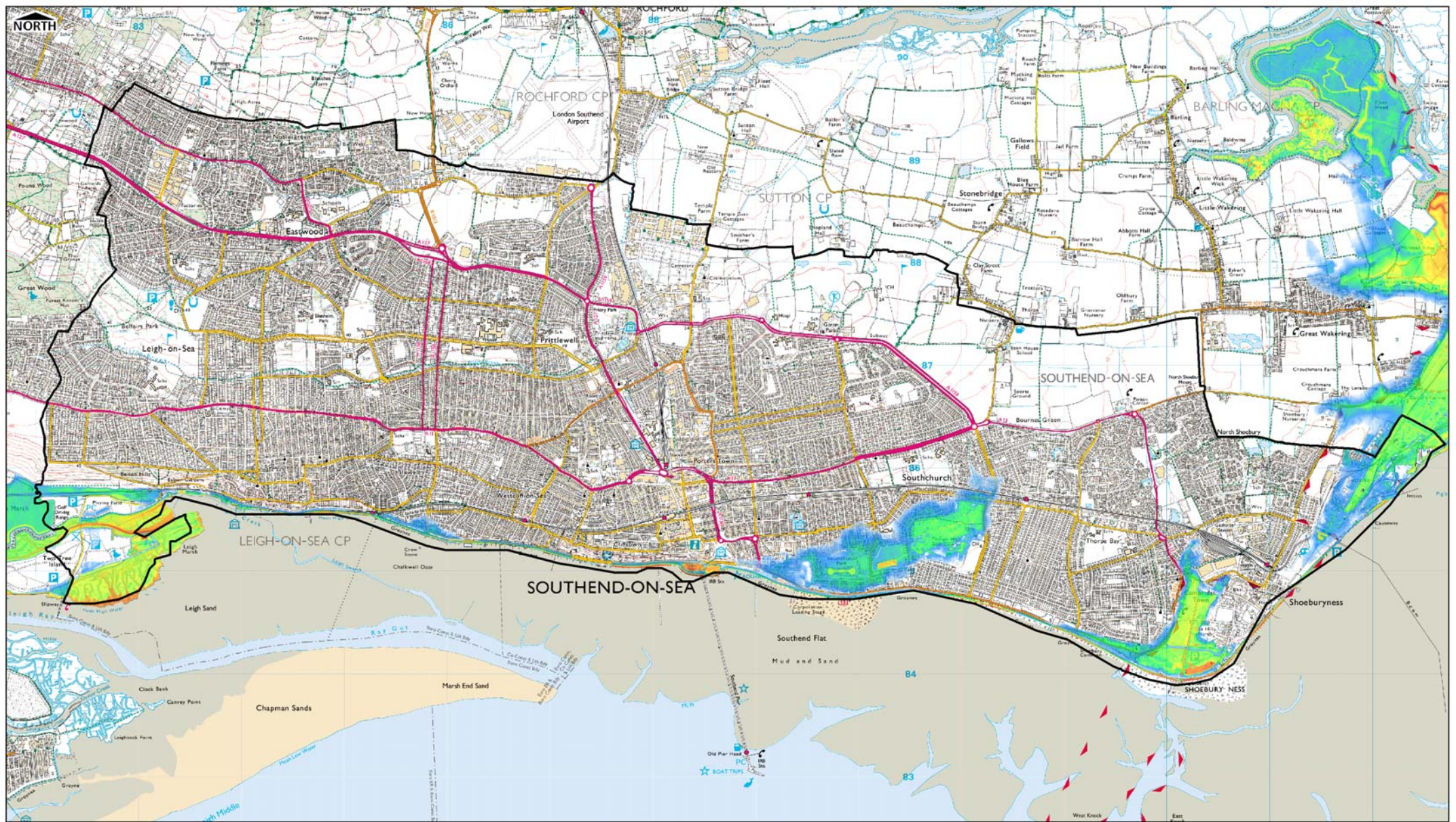
FIGURE C4 - COMPOSITE MAXIMUM FLOOD DEPTH 1000YR 2010 (BREACH AND OVERTOPPING)
