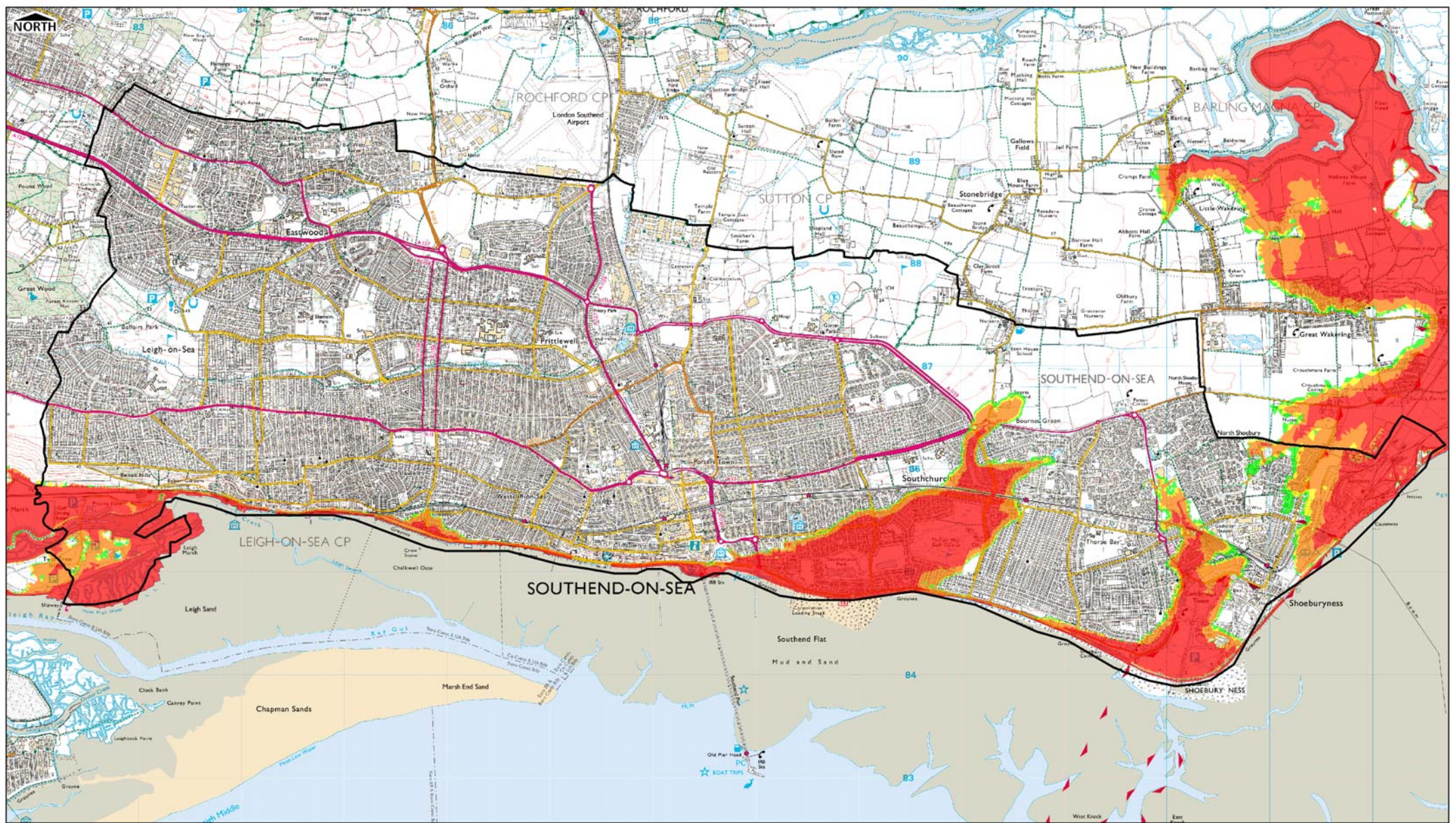
FIGURE C12 - COMPOSITE MAXIMUM HAZARD 1000YR 2110 (OVERTOPPING)
