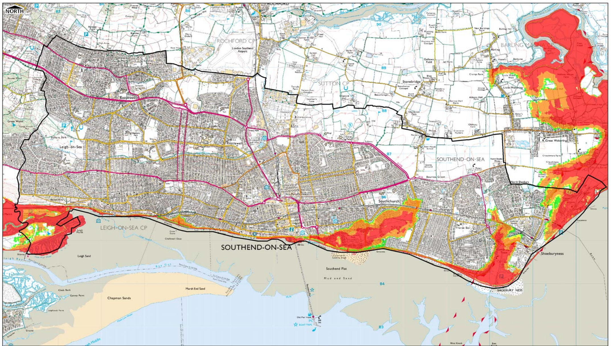
FIGURE C8 - COMPOSITE MAXIMUM HAZARD 200YR 2110 (BREACH AND OVERTOPPING)
