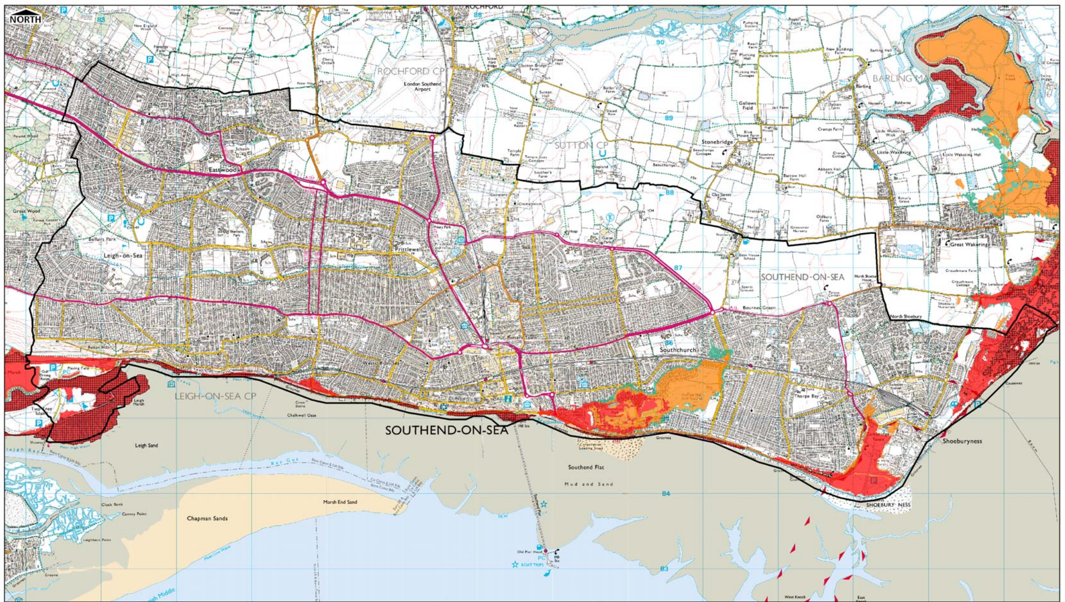
FIGURE C15 - COMPOSITE TIME TO INUNDATION (FROM BREACH EVENT) 1000YR 2010
