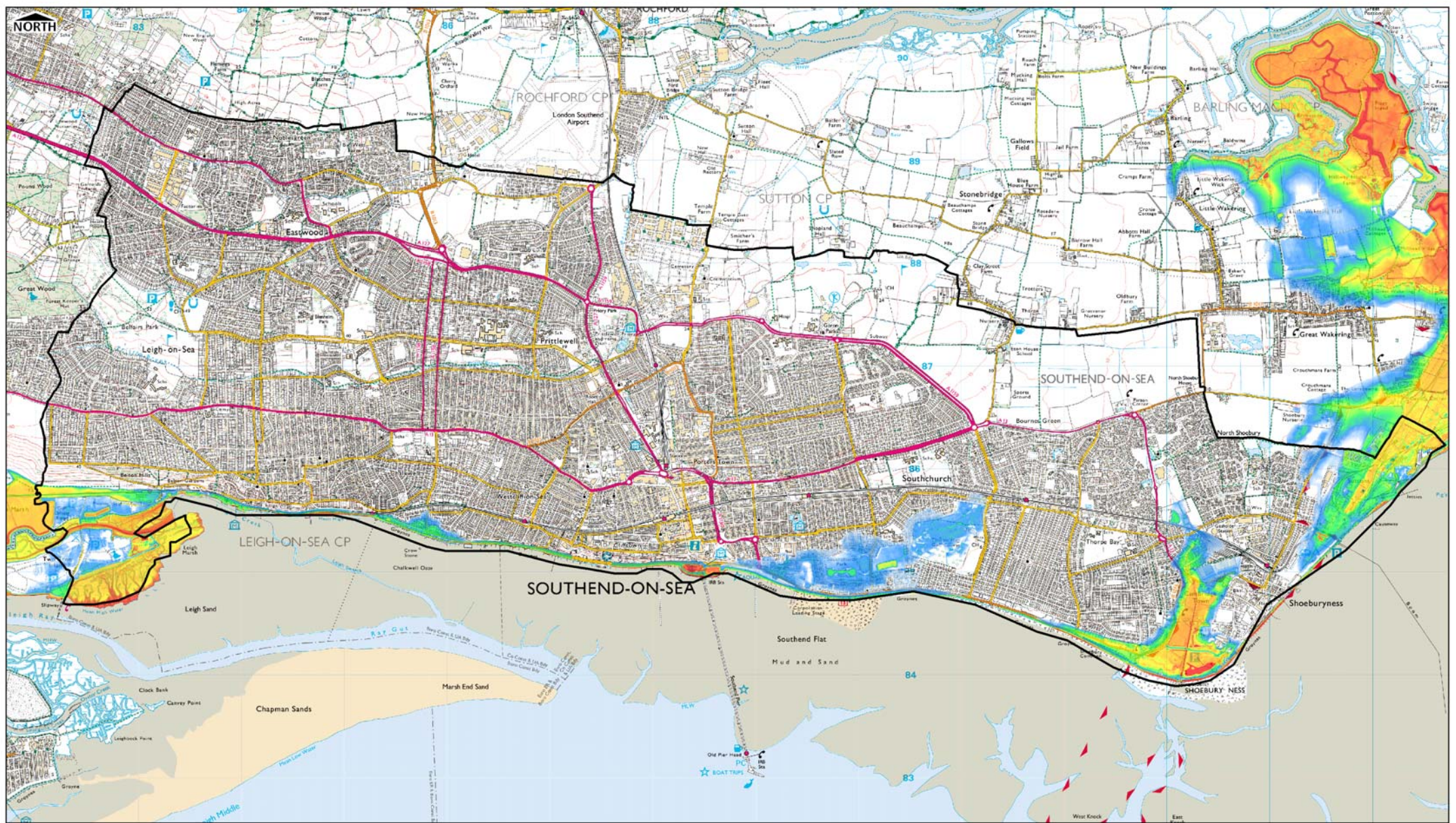
FIGURE C3 - COMPOSITE MAXIMUM FLOOD DEPTH 200YR 2110 (OVERTOPPING)
