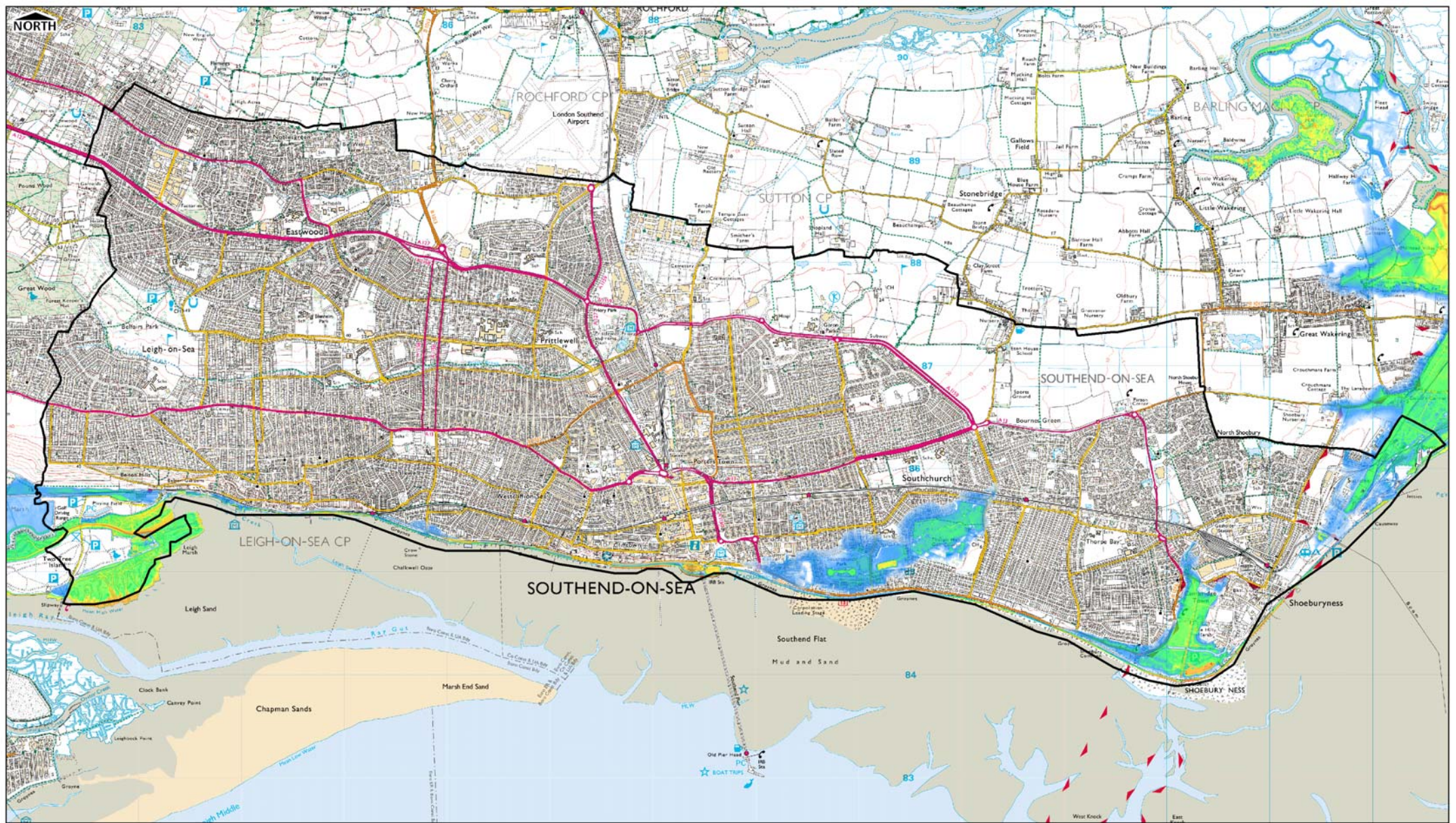
FIGURE C1 - COMPOSITE MAXIMUM FLOOD DEPTH 200YR 2010 (BREACH AND OVERTOPPING)
