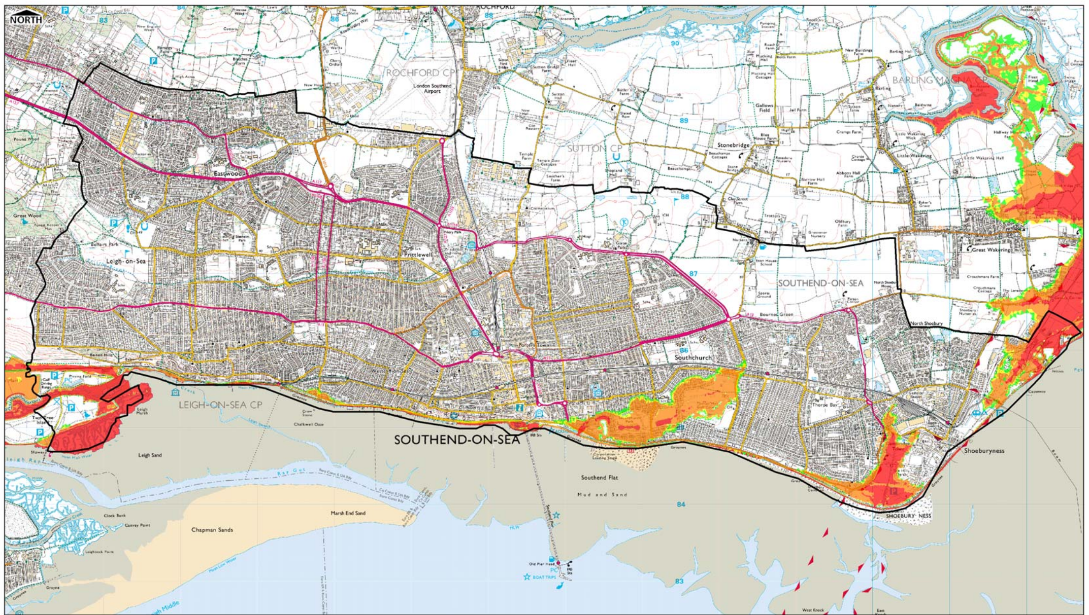
FIGURE C7 - COMPOSITE MAXIMUM HAZARD 200YR 2010 (BREACH AND OVERTOPPING)
